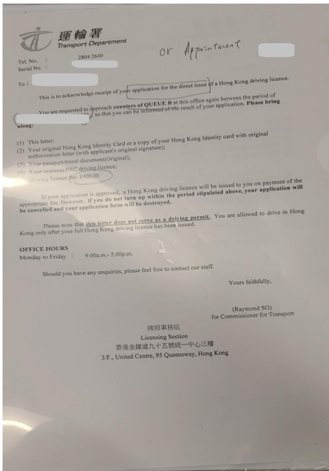
Acknowledge receipt
